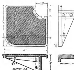
Figs. 2259-2262. Pilot Step, Atlantic (4-4-2) Locomotive. Pennsylvania Railroad.
